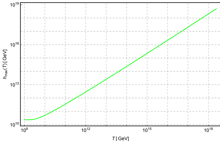
Figure : The position h_{\text{max}} of the local maximum separating two minima of the RG improved effective potential as a function of the temperature of thermal bath T .
