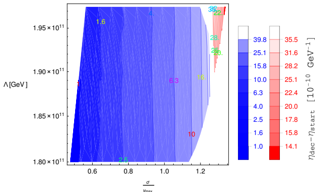
Figure : The dependence of the decay time of networks of Higgs domain walls as a function of the fraction \frac{\sigma}{h_{max}} and the suppression scale \Lambda for \eta_{start} = 10^{-10} \text{ GeV}^{-1} and standard deviation \sigma = 3.25 \times 10^{10} \text{ GeV} at initialization.
