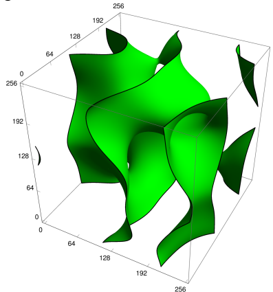
Figure : An example of the infinite network of domain walls.
